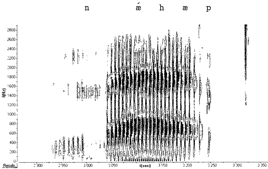
Figure 3-6 Plain alveolar nasal in 'he runs'
