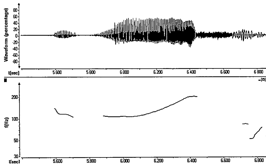
FIGURE 4-7. Waveform and pitch contour for 'my orange'
