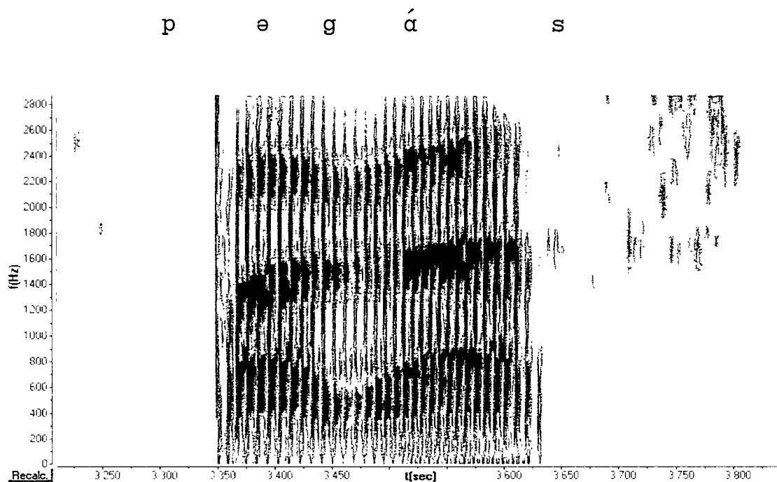
Figure 3-1 Spectrogram of a voiceless bilabial stop in 'cow'
