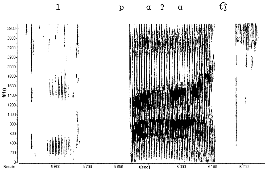
FIGURE 4-5. Spectrogram of a laryngeally ambiguous /a/ vowel for creaky voice in 'I help'
