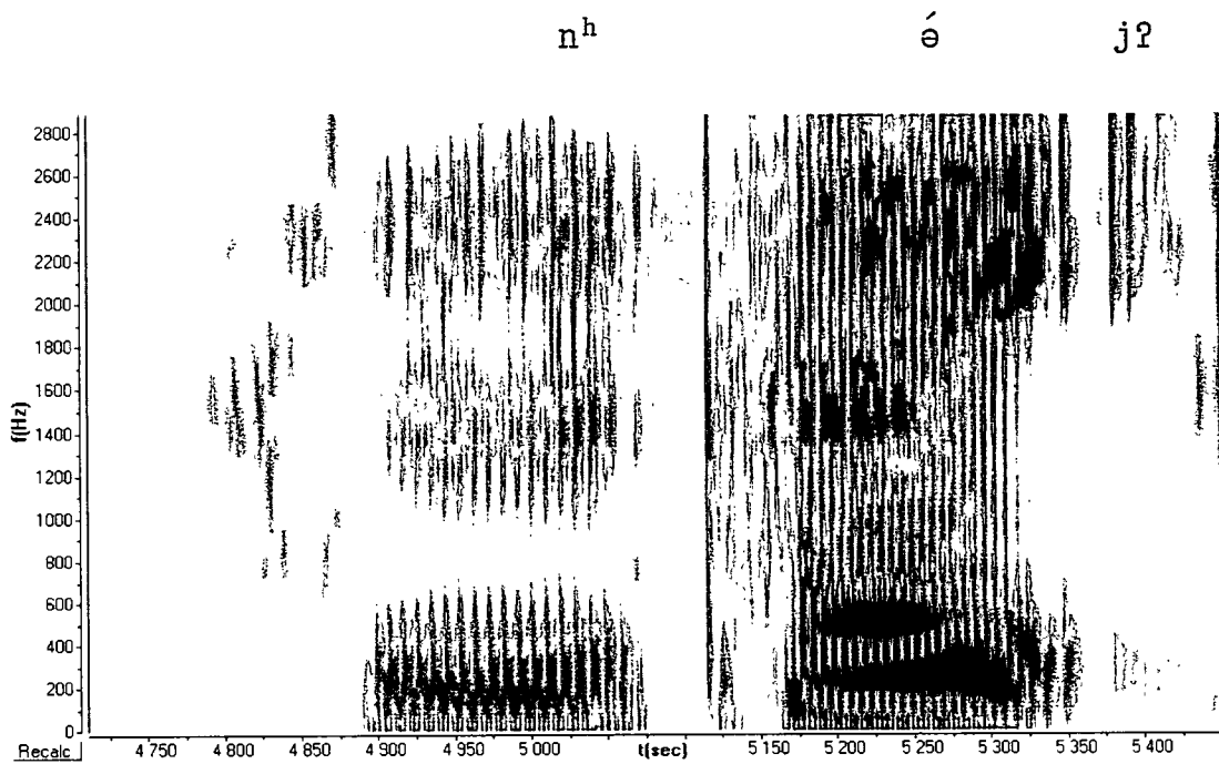
Figure 3-7 Post-aspirated alveolar nasal in 'he enters'
