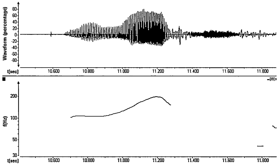
FIGURE 3-15. Waveform and pitch track for a high tone on 'your orange'.
