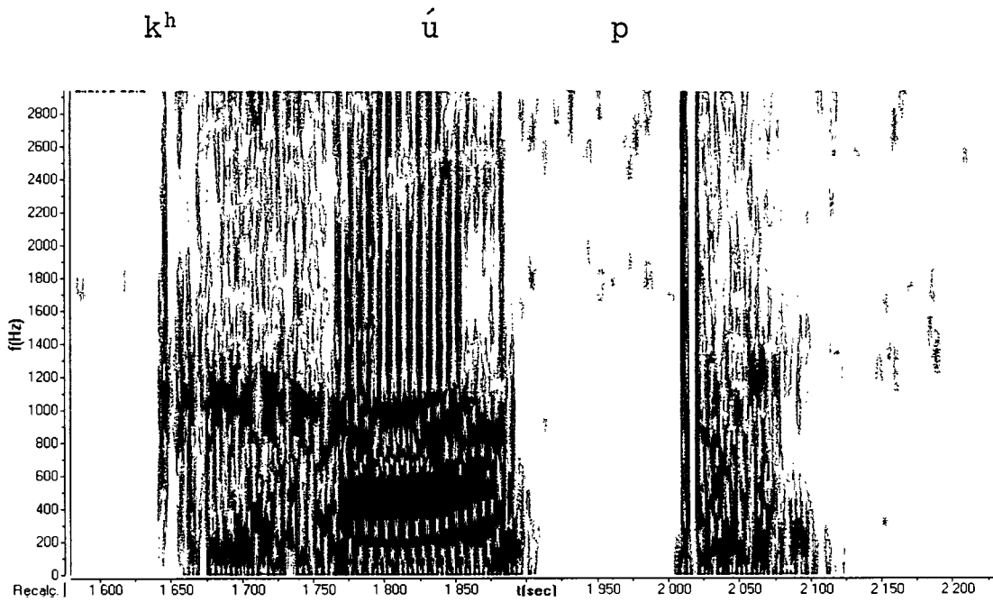
Figure 3-4 Aspirated velar stop in 'they reject him'
