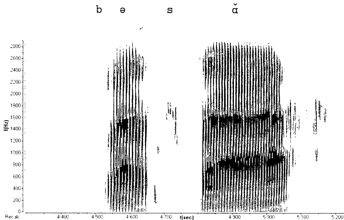
Figure 3-2 Spectrogram of a voiced bilabial stop in 'ears of corn'
