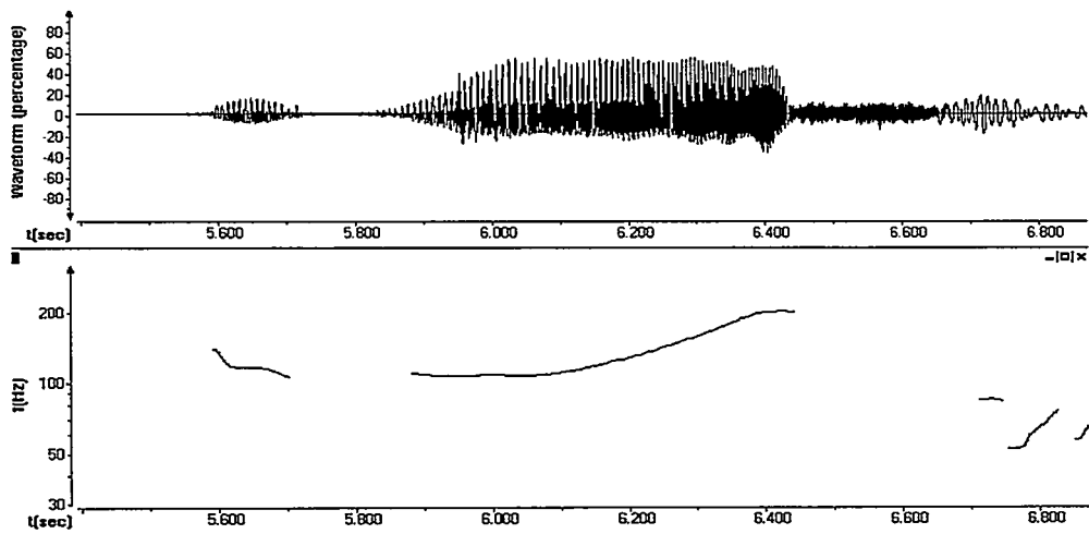
FIGURE 3-16. Waveform and pitch track for a low (rising) tone in 'my orange'.
