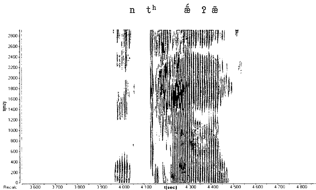
FIGURE 3-14. Spectrogram of a nasal vowel in 'tamale'
