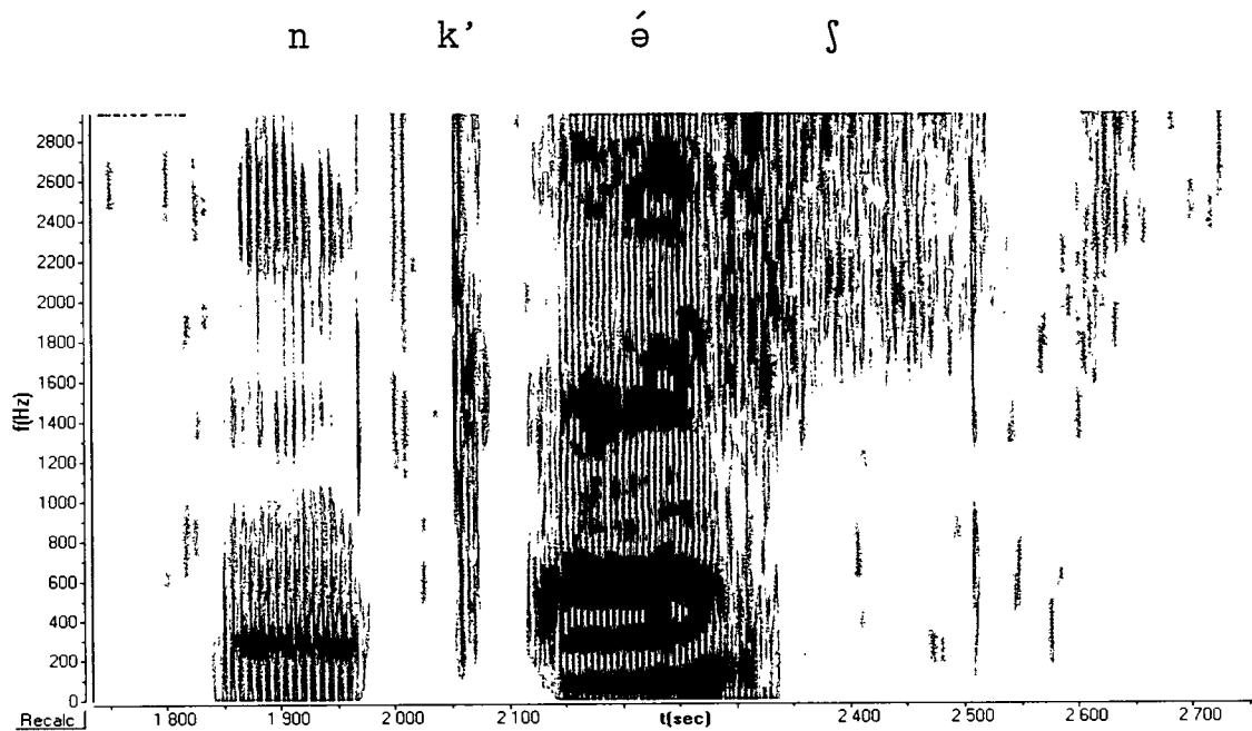
Figure 3-5 Glottalized velar stop in 'piece of paper'
