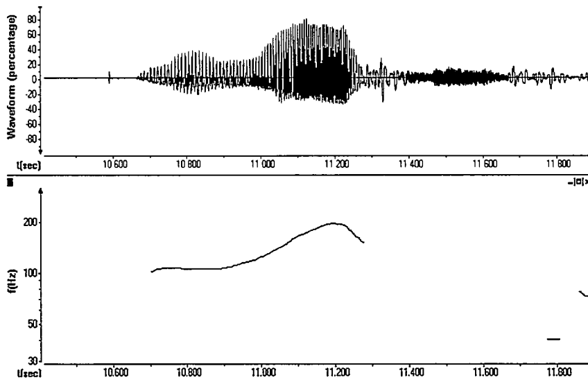
FIGURE 4-6. Waveform and pitch contour for 'your orange'
