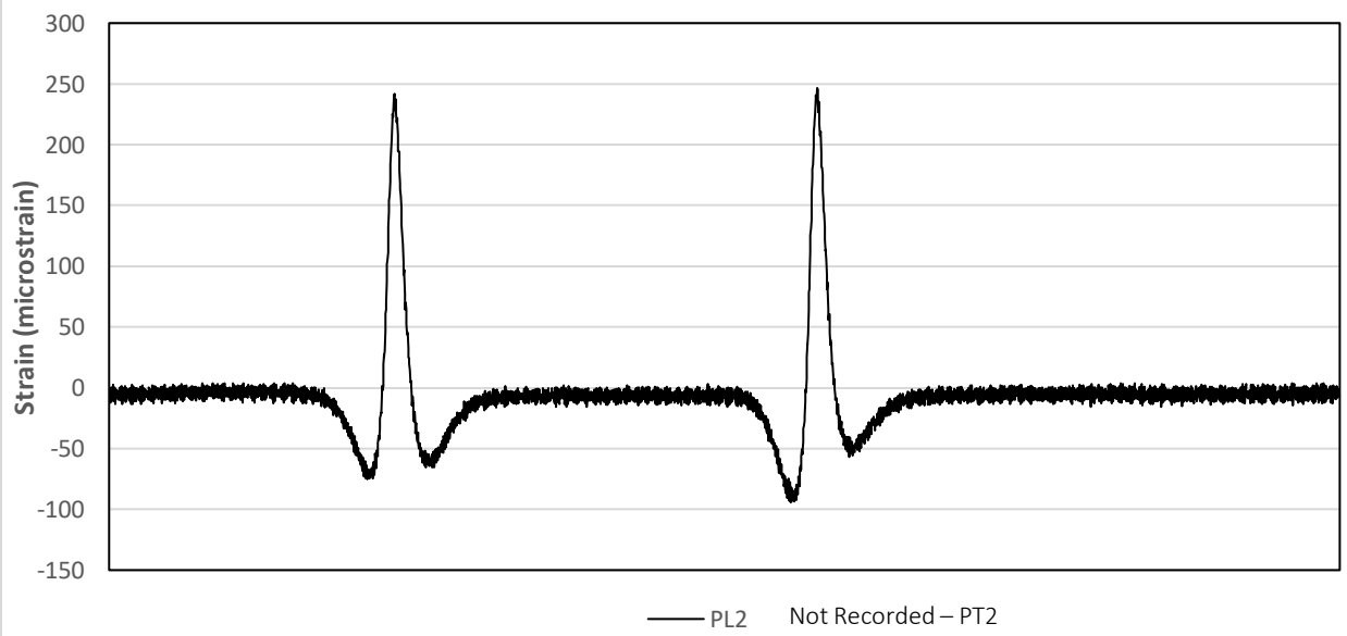
Figure D2-6 Strain Signals Recorded by PL2 – 0 Passes
