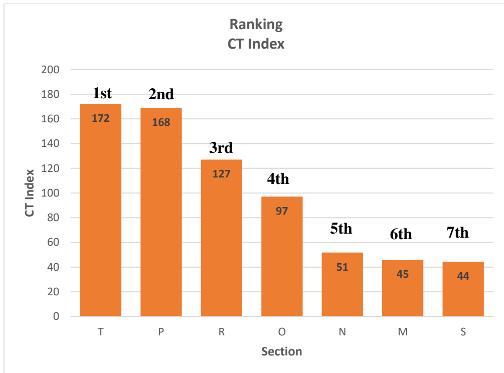
Figure 4.42 Ranking of the CT_{INDEX} values -IDEAL-CT Test
