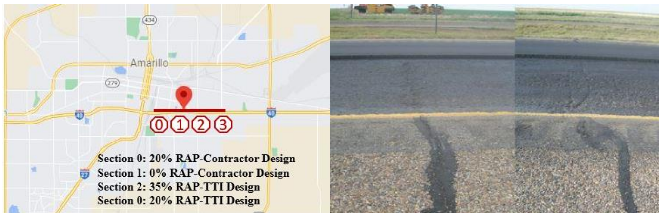
Figure 2.19 I-40 Experimental sections. Location and existing pavement condition after 4” milling, Zhou et al., (2011)
