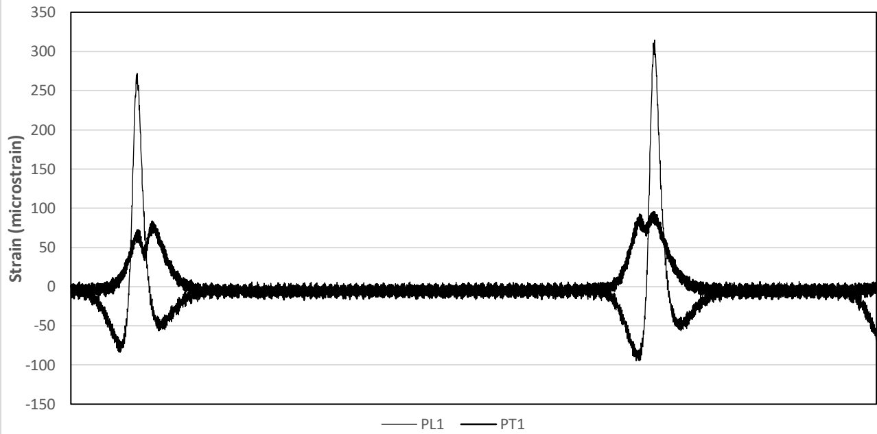
Figure D2-5 Strain Signals Recorded by PL1 and PT1 – 0 Passes
