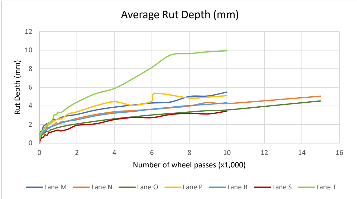
Figure 4.6 Average central rut depth for all mixes
