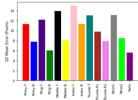
Figure 6: Per-joint mean 2D error. T and R denote tip and root respectively (e.g. Index-T denotes the tip of the index finger)
