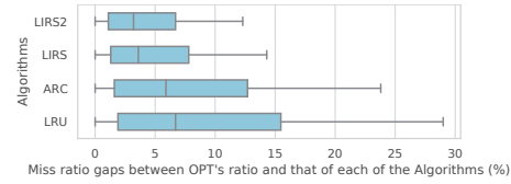
Figure 7: Miss ratio gaps between OPT’s ratio and that of an algorithm under test. For each of the algorithms, 2,300 miss ratios are collected (for each of the 115 traces on 20 cache sizes evenly distributed between 1% of the data set size and the size where the miss ratio starts to plateau out). For each algorithm, a box plot has lines corresponding to first quartile, median, and third quartile. Lines extending from a box indicate minimum and maximum.
