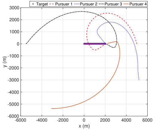
(a) Pursuer planar trajectories
