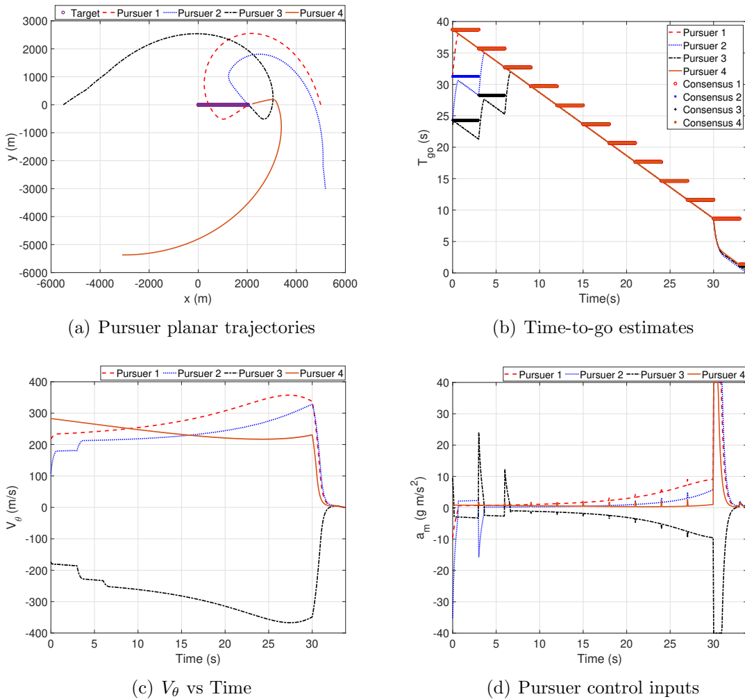
Figure 3.9. Directed cycle Constant Velocity target: Trajectory, time-to-go estimates, V_\theta vs time and control inputs.
