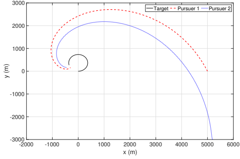
(a) Pursuer planar trajectories
