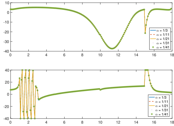
(b) a_{m,i} sensitivity to \alpha
