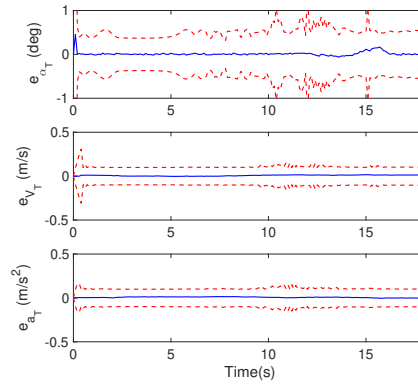
(b) UKF target state errors: Pursuer 2
