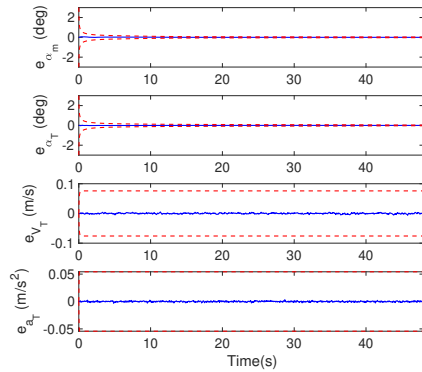
(f) Pursuer 2: Errors in States \alpha_m, \alpha_T, V_T, a_T
