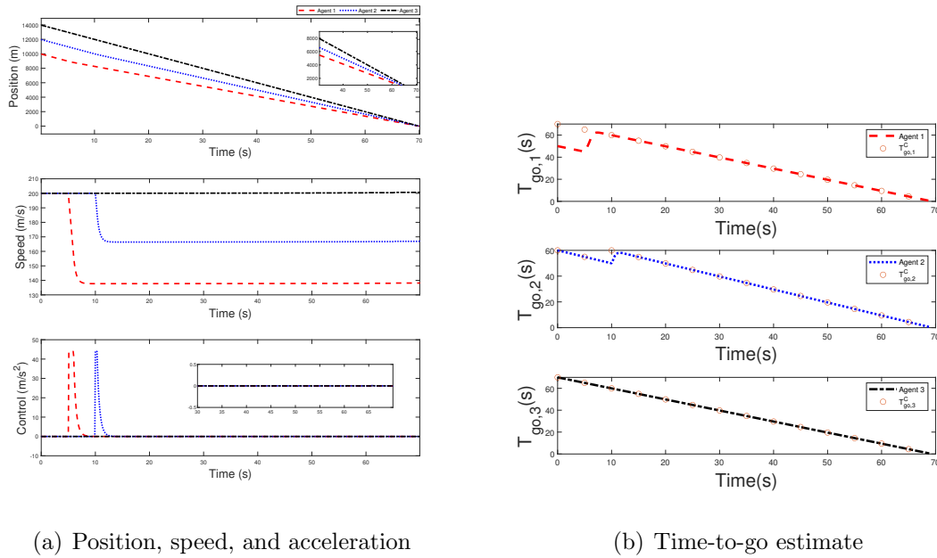
Figure 2.7. Max-time protocol results (three agents).
