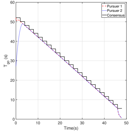
(b) Time-to-go estimates
