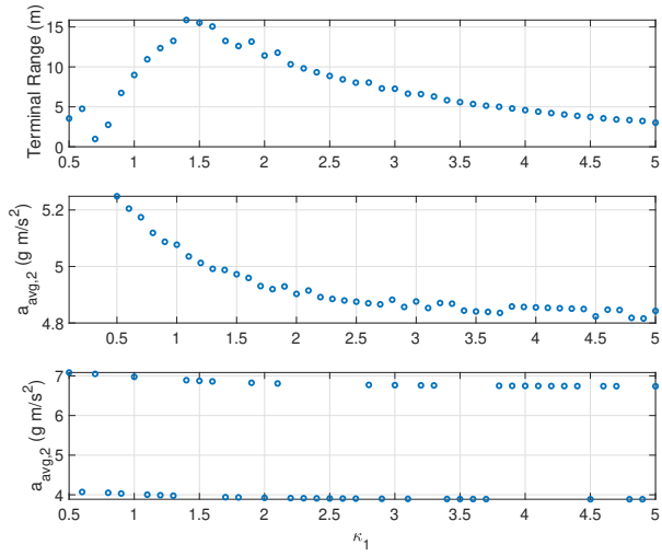
(a) Average performance vs \kappa_{i,1}
