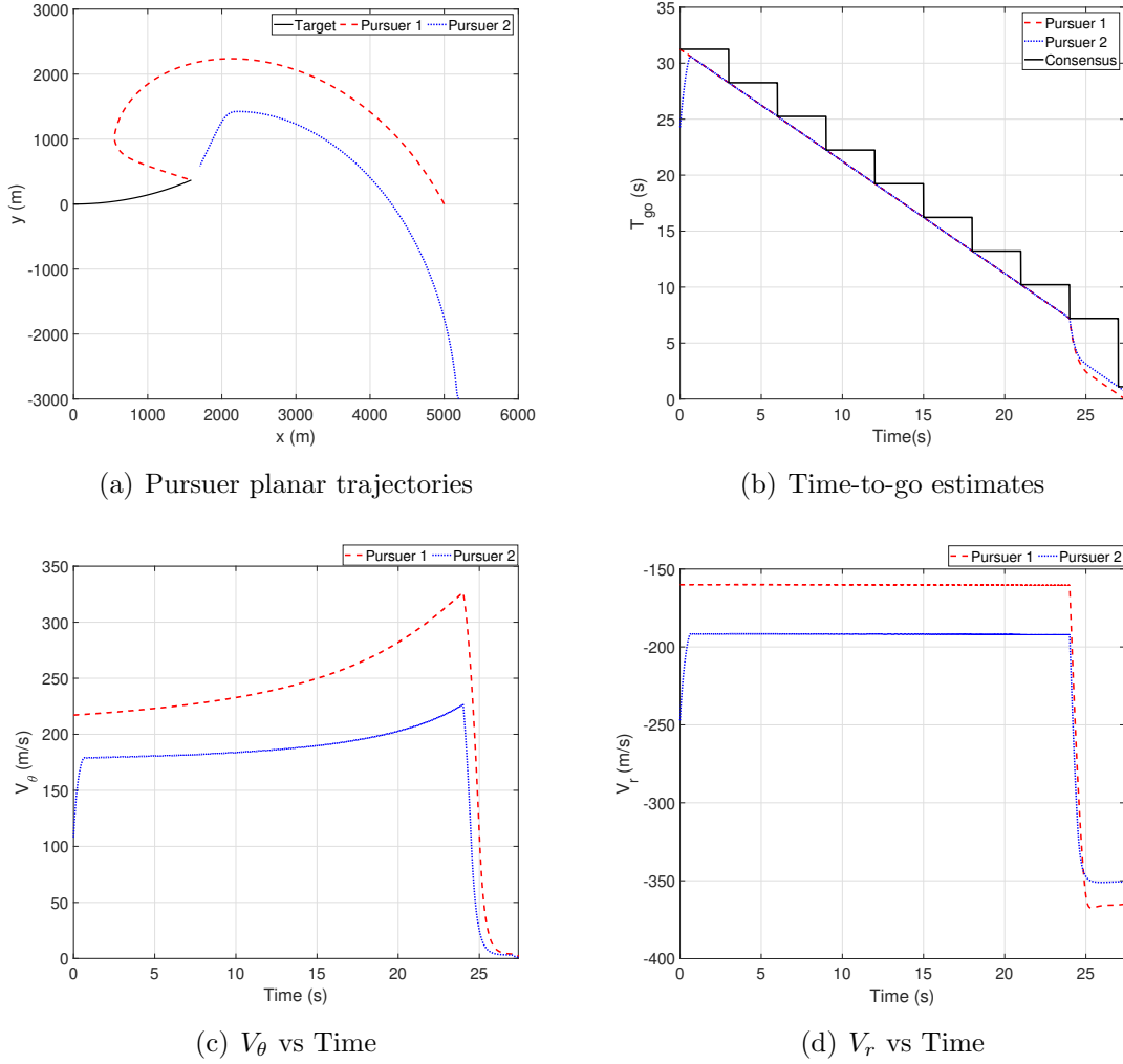
Figure 3.13. Maneuvering target: Trajectory, time-to-go estimates, V_\theta and V_r vs time.
