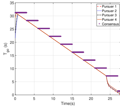
(b) Time-to-go estimates
