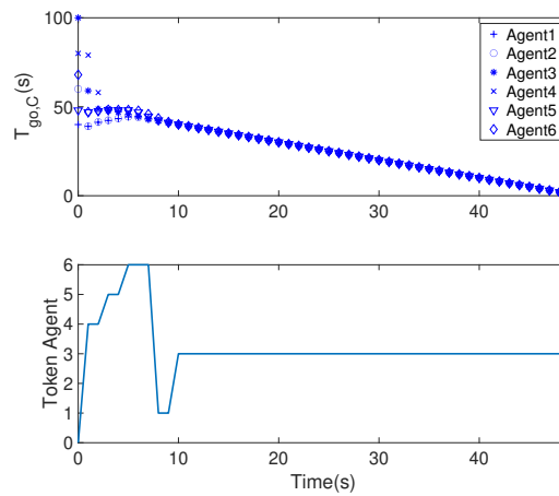
Figure 2.13. Tokenized achievable-time protocol consensus time-to-go and token agents vs time.
