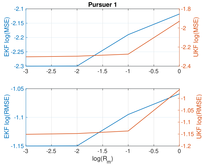
(a) Pursuer 1 estimation errors
