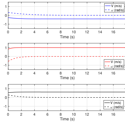
(b) Control Inputs
