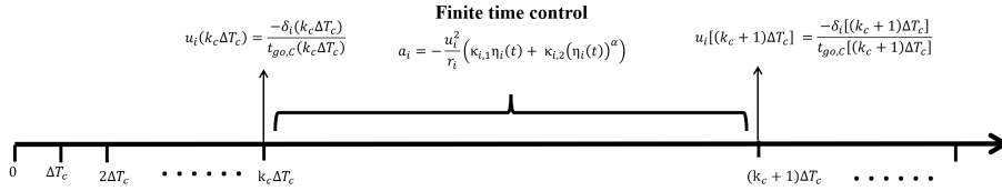
Figure 2.2. Continuous-discrete framework of consensus.
