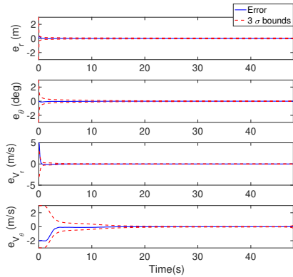
(e) Pursuer 2: Errors in States r, \theta, V_r, V_\theta
