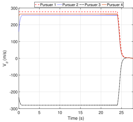
(c) V_\theta vs Time
