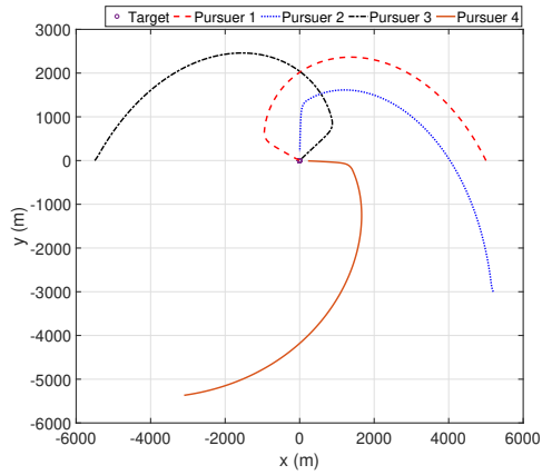
(a) Pursuer planar trajectories
