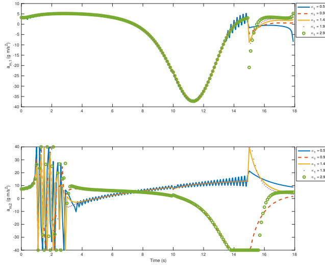
(b) a_{m,i} sensitivity to \kappa_{i,1}
