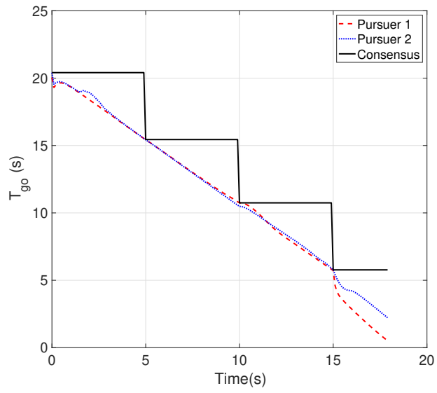
(b) Time-to-go estimates
