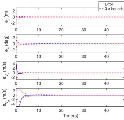
(c) Pursuer 1: Errors in States r, \theta, V_r, V_\theta
