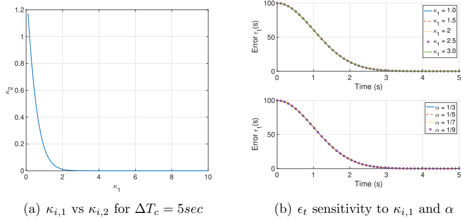
Figure 3.2. t_{go,C} convergence plots.
