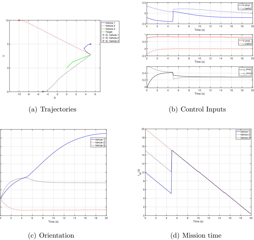
Figure 4.5. Max time: Heterogeneous multi vehicle optimal rendezvous.
