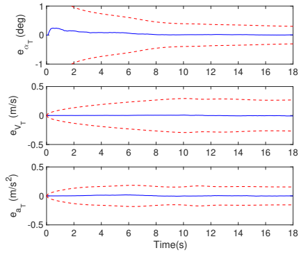
(c) EKF target state errors: Pursuer 1
