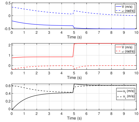
(b) Control Inputs
