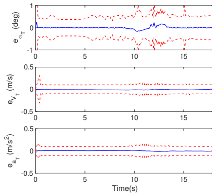
(a) UKF target state errors: Pursuer 1
