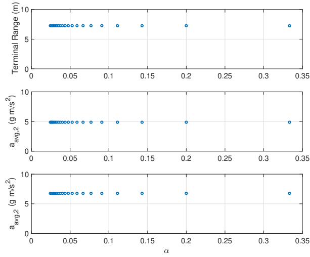
(a) Average performance vs \alpha
