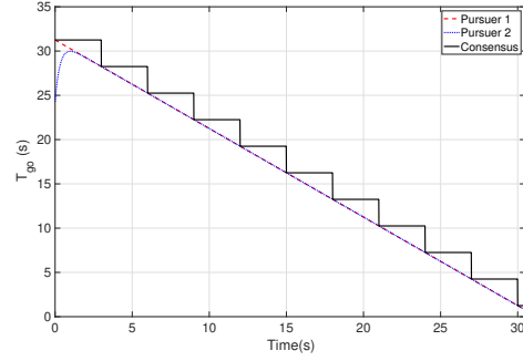
(b) Time-to-go estimates
