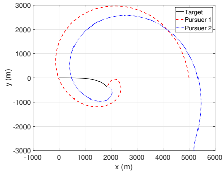
(a) Pursuer trajectories
