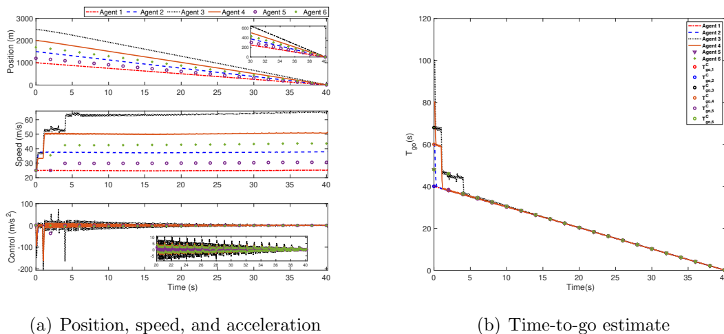
Figure 2.11. Min-time protocol results (six agents).
