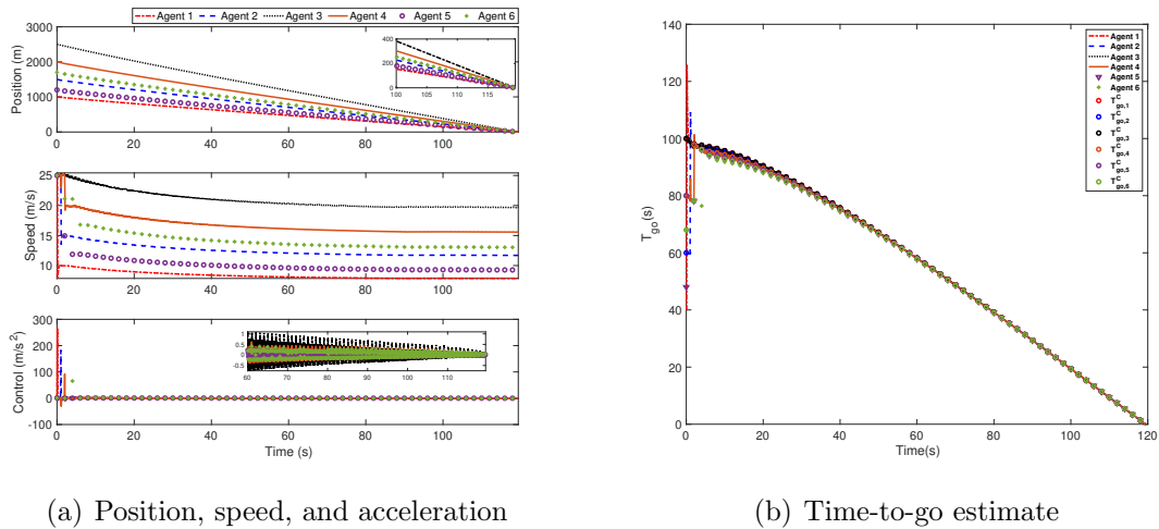
Figure 2.10. Max-time protocol results (six agents).
