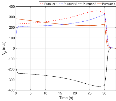
(c) V_\theta vs Time
