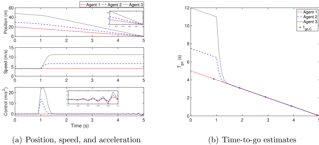
Figure 2.4. Min-time protocol results.
