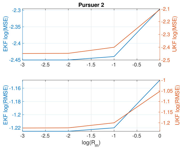
(b) Pursuer 2 estimation errors
