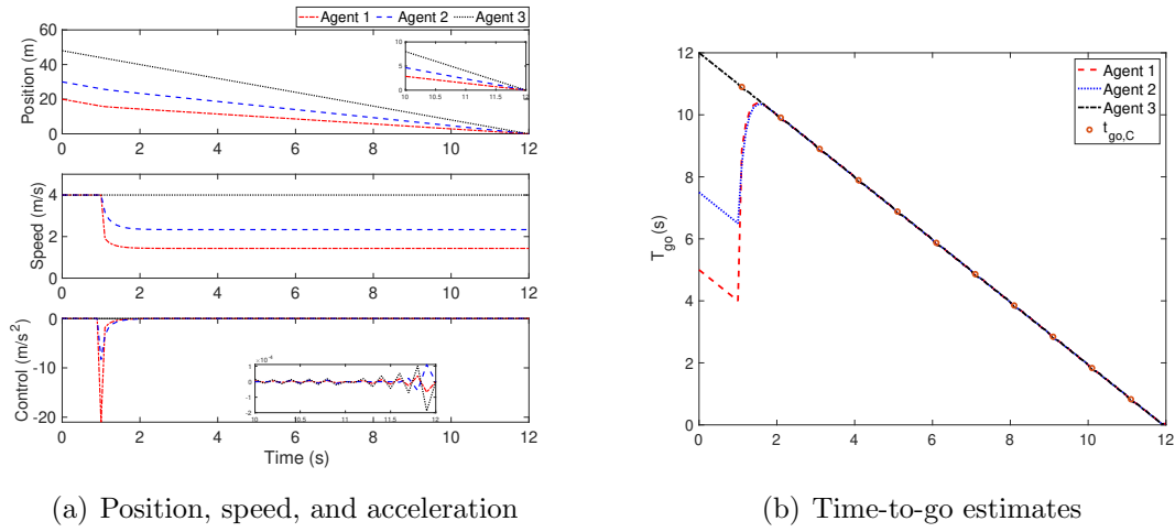
Figure 2.3. Max-time protocol results.
