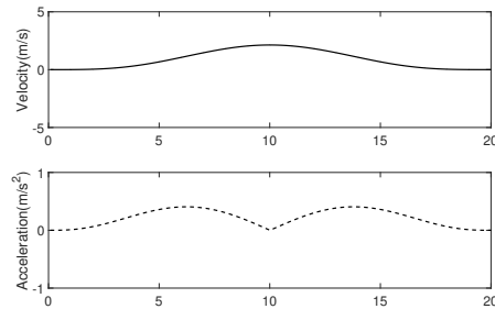
(e) Quadrotor Approach
