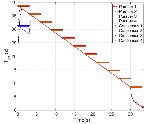
(b) Time-to-go estimates
