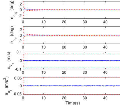
(d) Pursuer 1: Errors in States \alpha_m, \alpha_T, V_T, a_T
