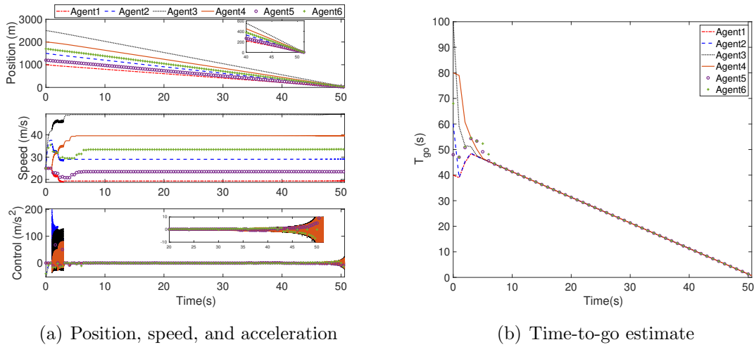
Figure 2.12. Tokenized achievable-time protocol results (six agents).
