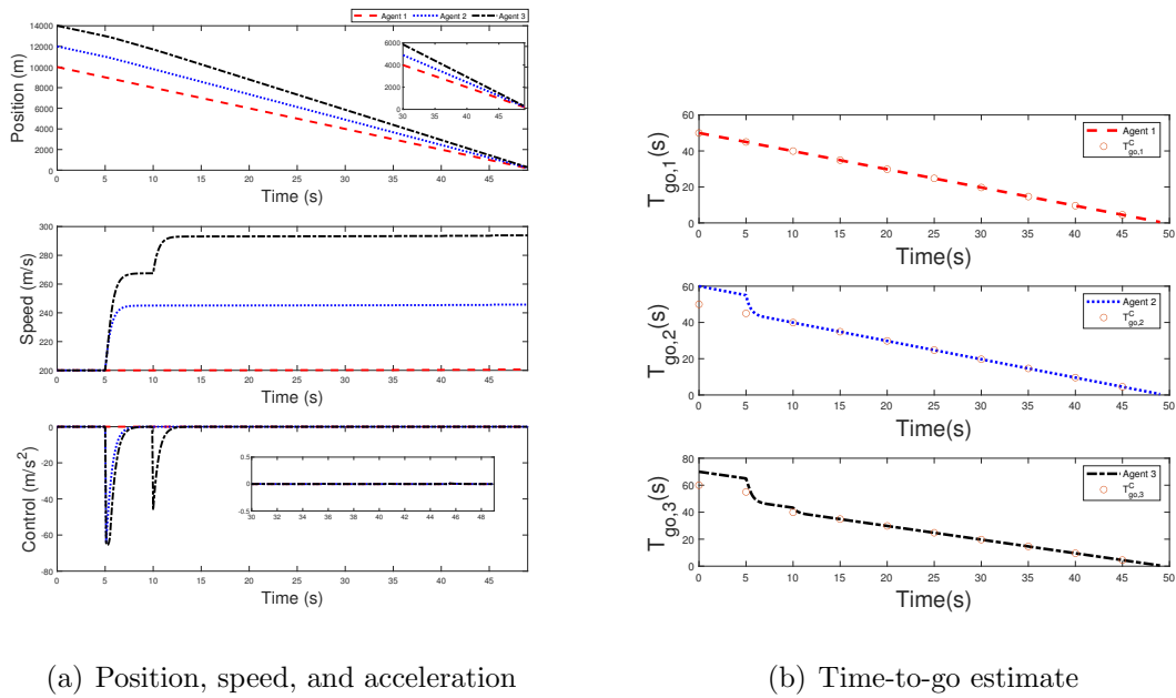
Figure 2.8. Min-time protocol results (three agents).
