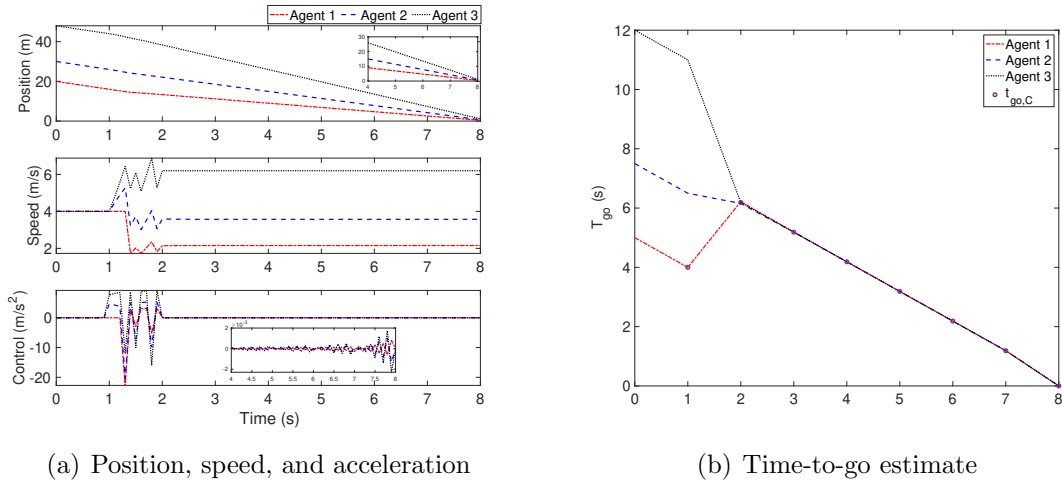
Figure 2.5. Achievable-time protocol results.
